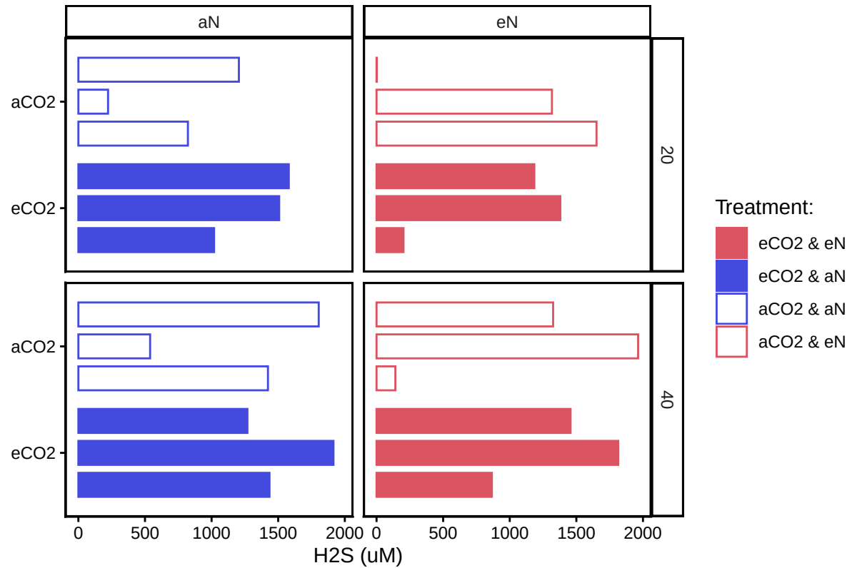
CO2xNxPhrag: Porewater Sulfide
